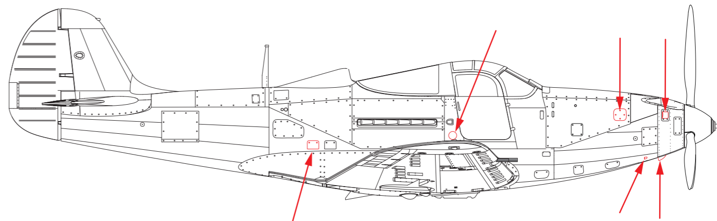
P-39 D Airacobra diagram of necessary modifications
